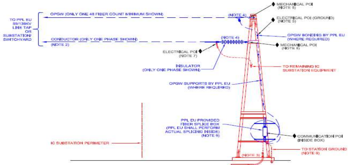
SUBSTATION DEADEND INTERCONNECTION POINT DIAGRAM WITH OPGW
