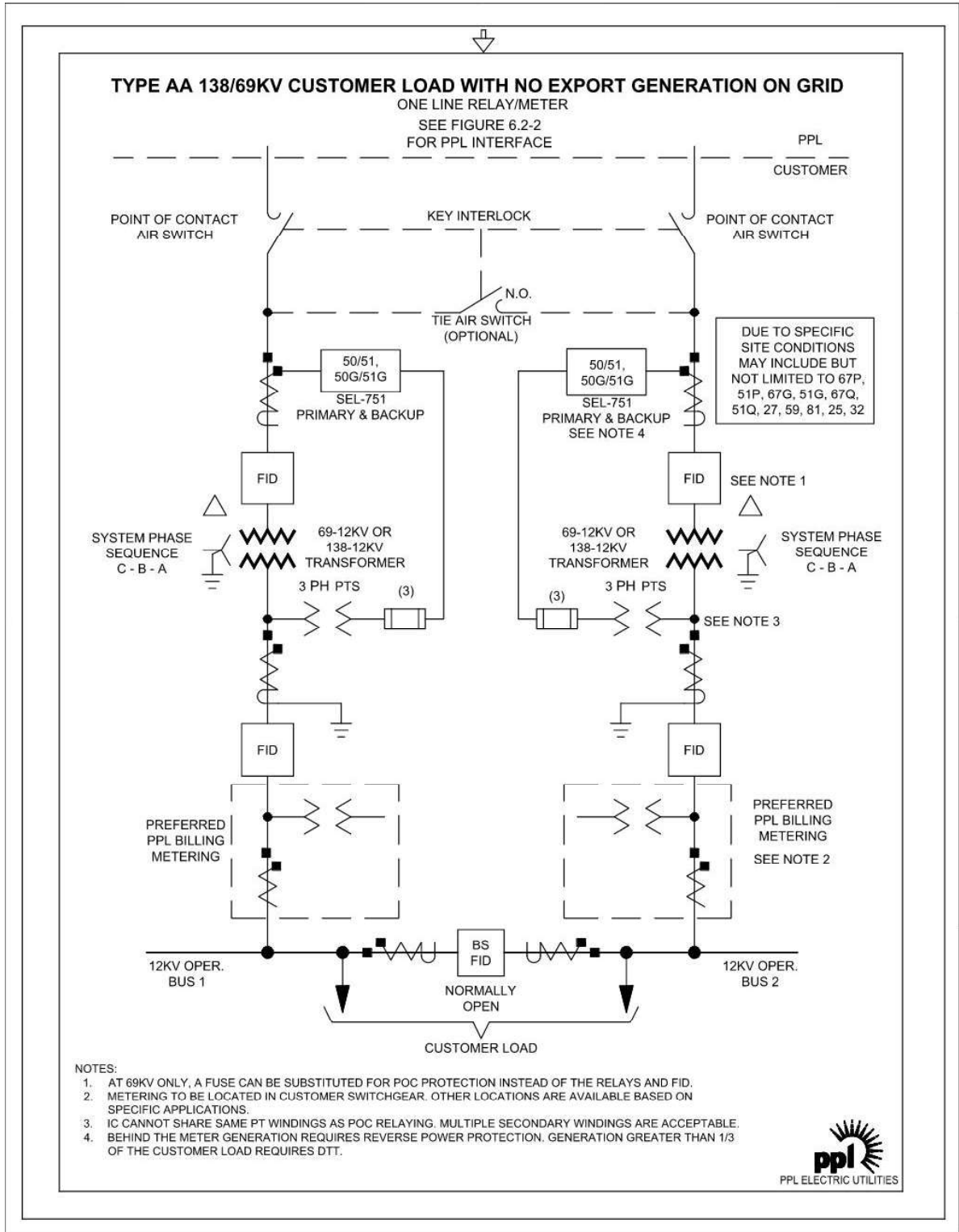
Figure 12.3.3.9-1 – Type "AA" Customer Configuration
