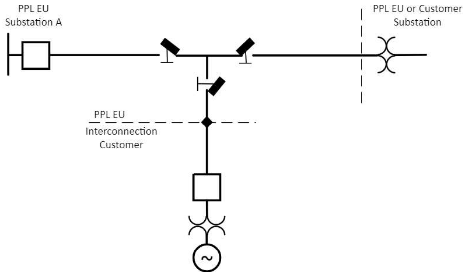
Figure 5.2-1 – Example line tap configuration connected to Generation Facilities
