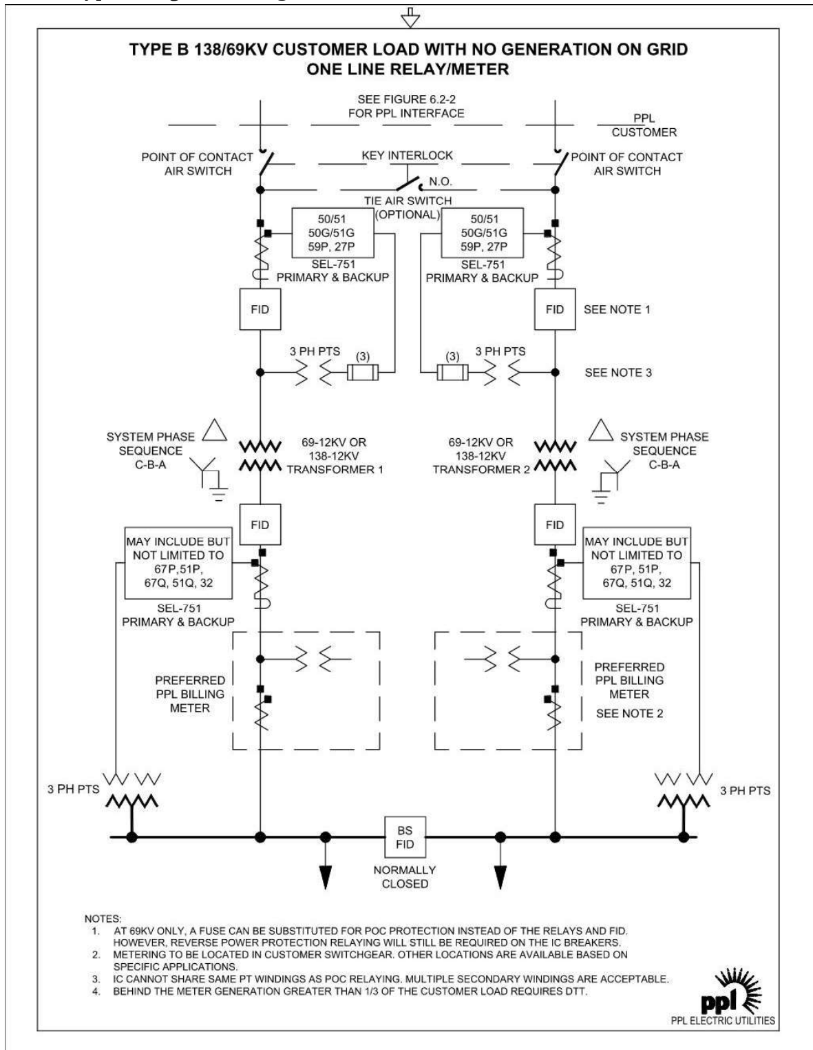
Figure 12.3.4.11-1 – Type "B" Customer Configuration
