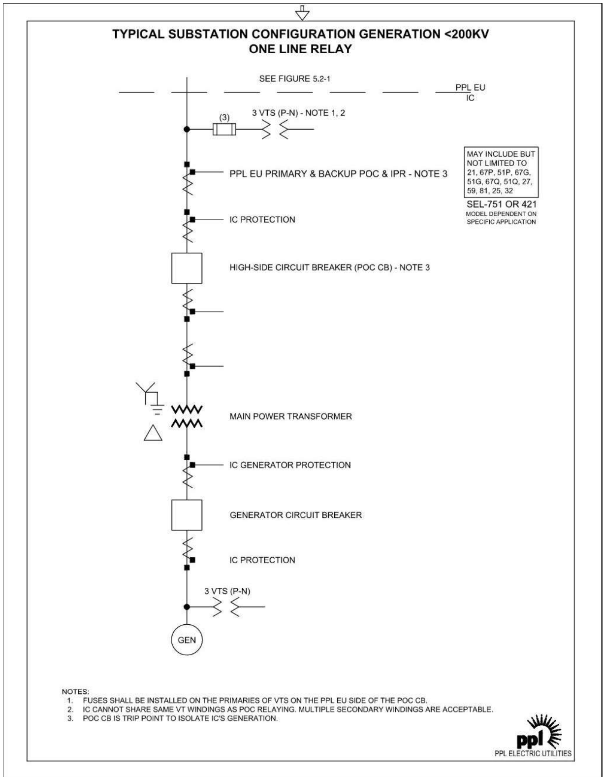
Figure 12.4.2.-2 Typical IC Generation Installation <200kV
