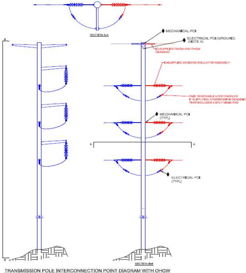
Figure 2: Point of Interconnection at a PPL EU Transmission Structure (with OHGW)
