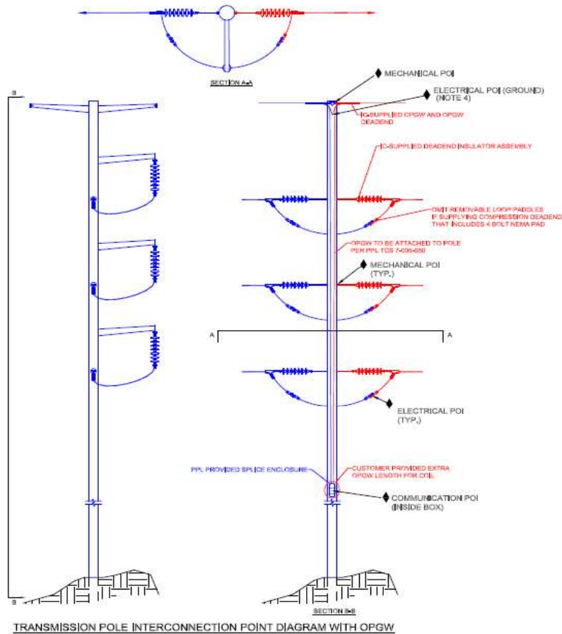
Figure 1: Point of Interconnection at a PPL EU Transmission Structure (with OPGW)
