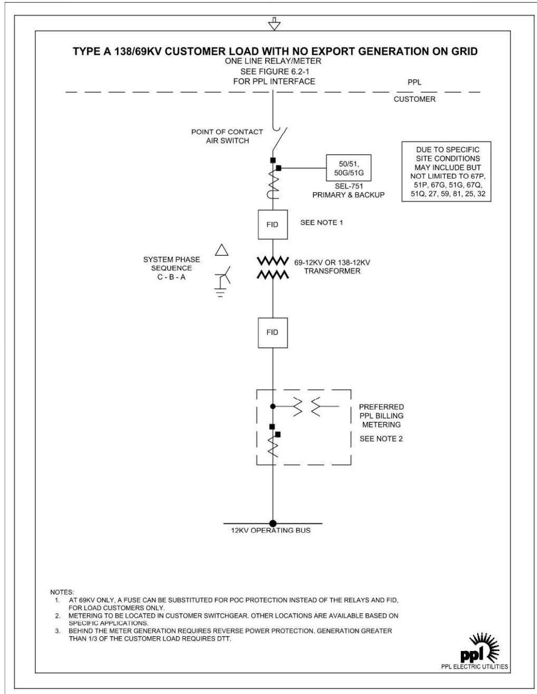
Figure 12.3.2.10-1 – Type "A" Customer Configuration.
