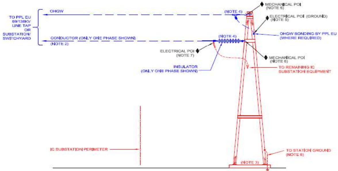
SUBSTATION DEADEND INTERCONNECTION POINT DIAGRAM WITH OHGW
