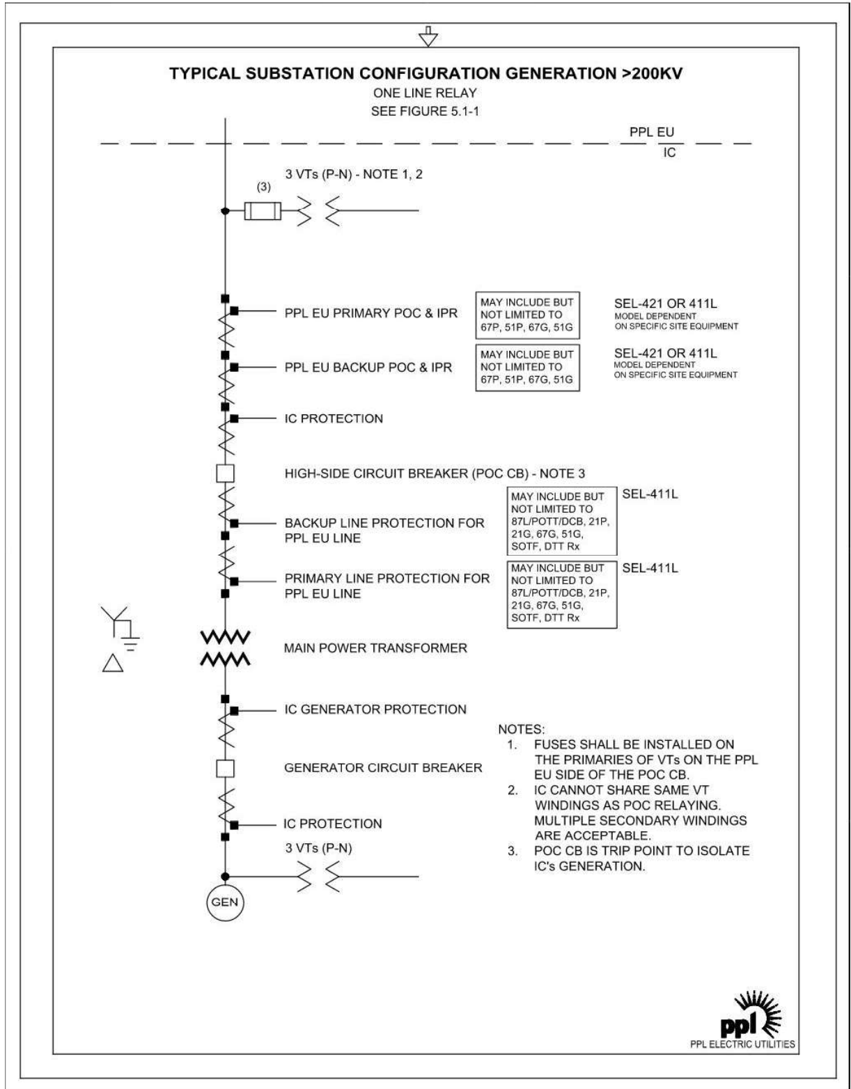
Figure 12.4.2.-1 Typical IC Generation Installation >200kV
